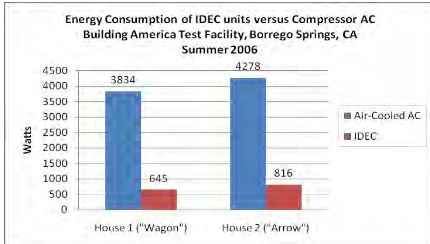
Figure 2: Comparison of Energy Use of IDEC units versus compress AC, Borrego Springs, CA
