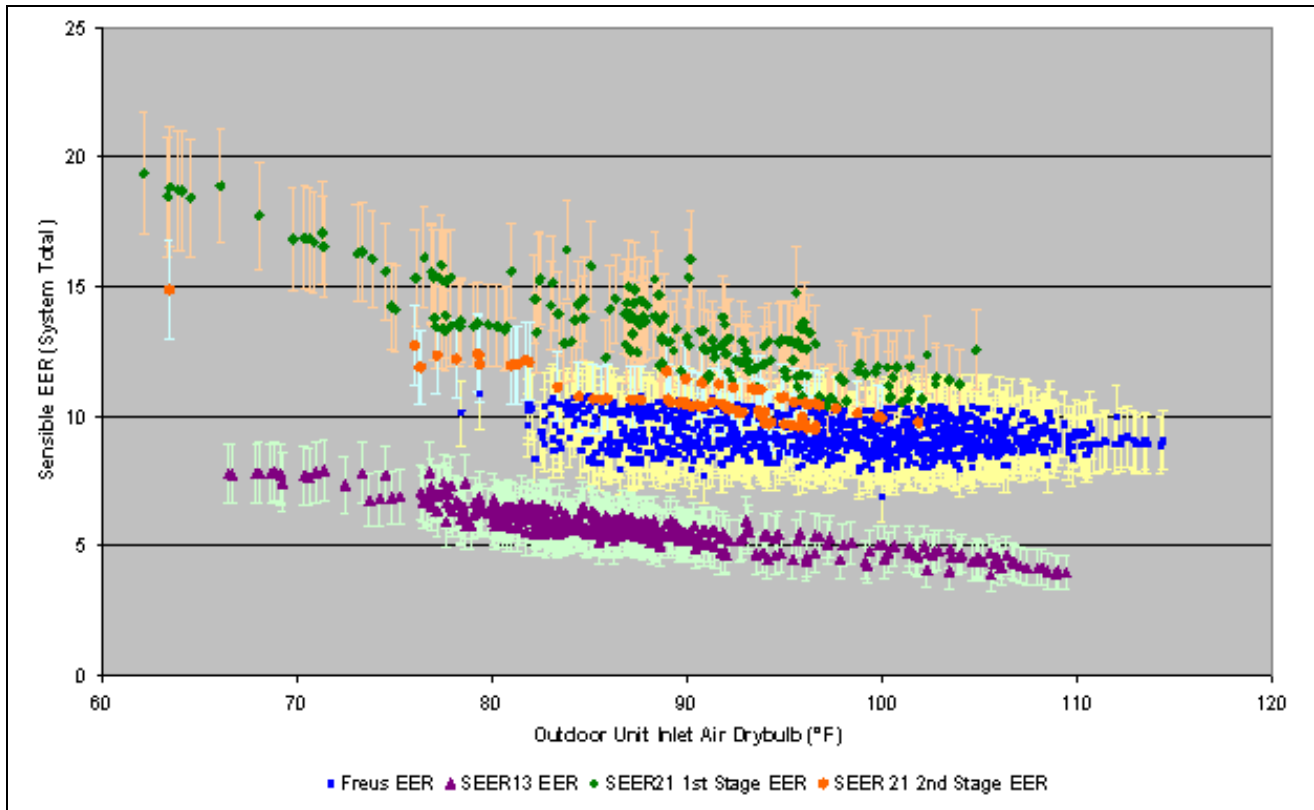
Figure 4. Evaporative-condensers are 40-50% more efficient at delivering cooling on hot days than SEER 13 system vapor-compression technologies, and provide equivalent performance to the SEER 21, which is the most advanced vapor-compression technology currently available in the marketplace.
