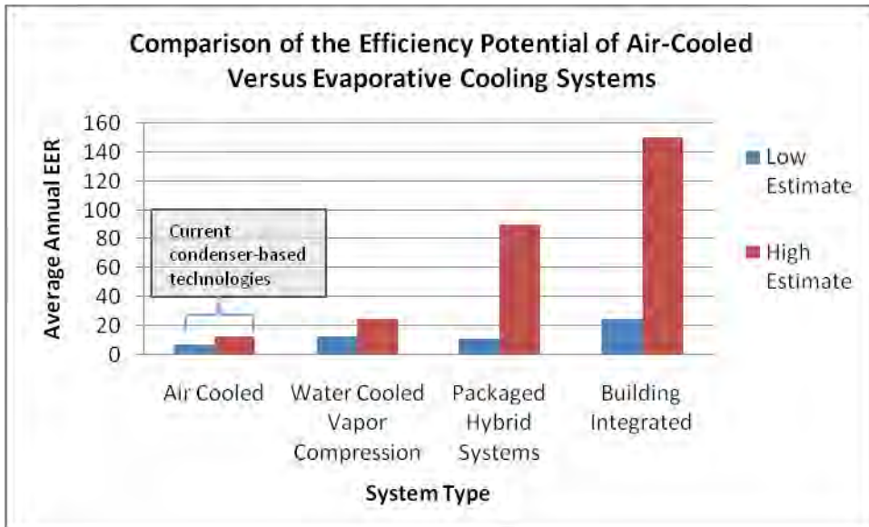
Figure 1: Comparison of the Average Annual EER of Vapor-Compression and Evaporative Cooling System Technologies
